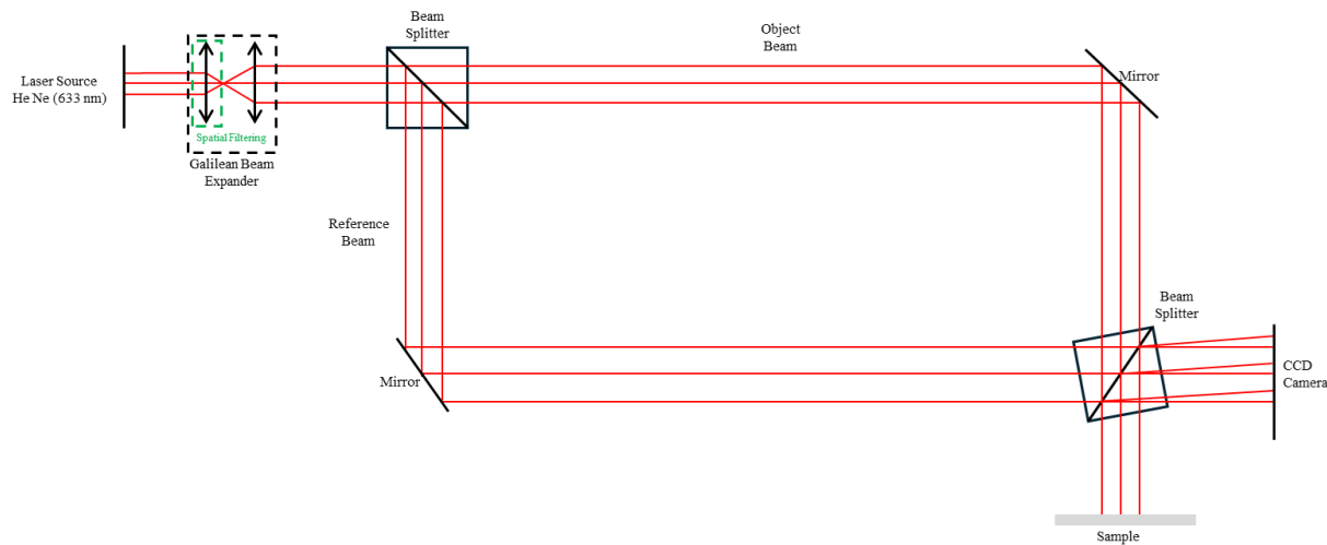
Figure 1. Reflection-mode DH optical system layout.
